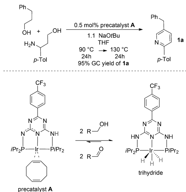
Scheme 2. Optimized reaction conditions (top) and formation of the catalyst resting state (trihydride, bottom right).
